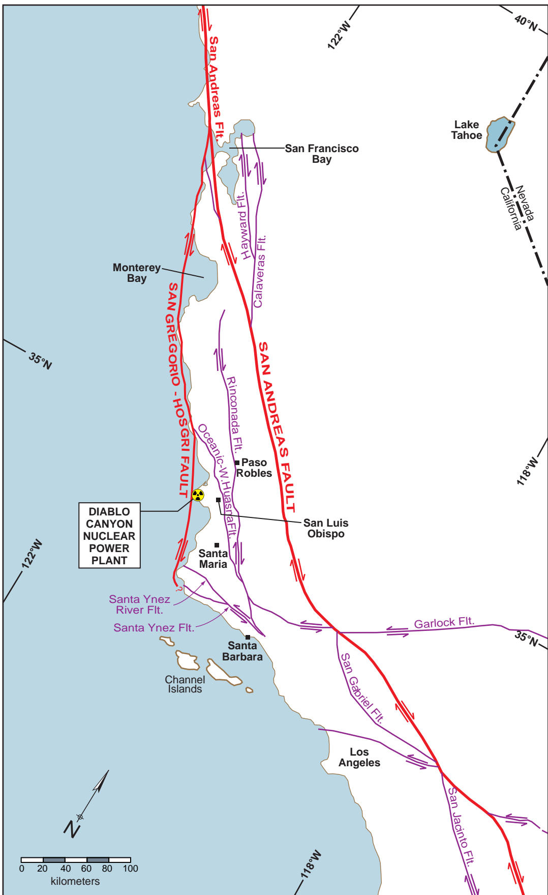
Major Faults Associated with the San Andreas Fault Zone (from Dickinson, GSA Spec. Paper, 2005)
